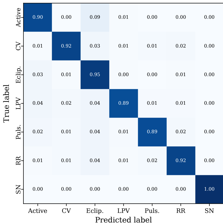
(c) LSTM
